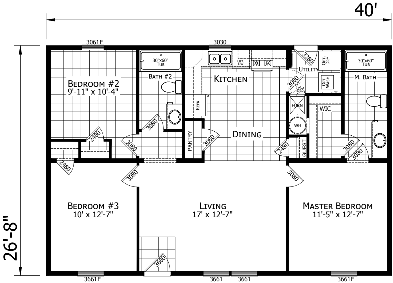
MODEL 122-A-34025 3 BEDROOM 2 BATH 40'-0" x 26'-8" 1067 Sq. Ft. TOTAL 06-03-21
